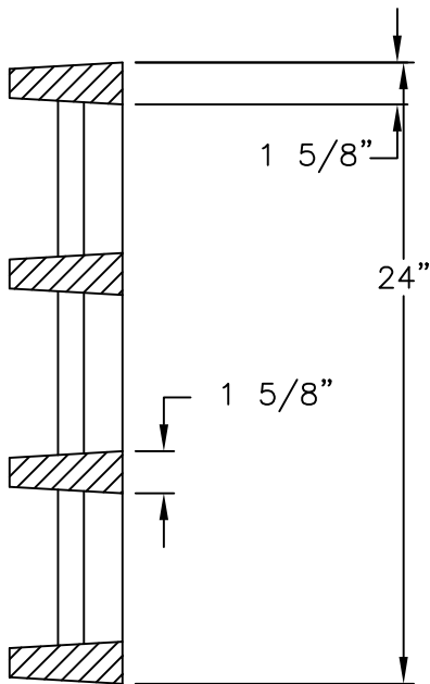
GRATE SECTION
