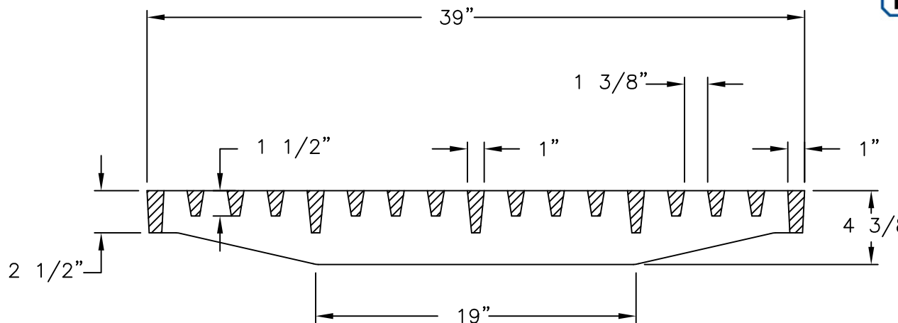
GRATE SECTION
